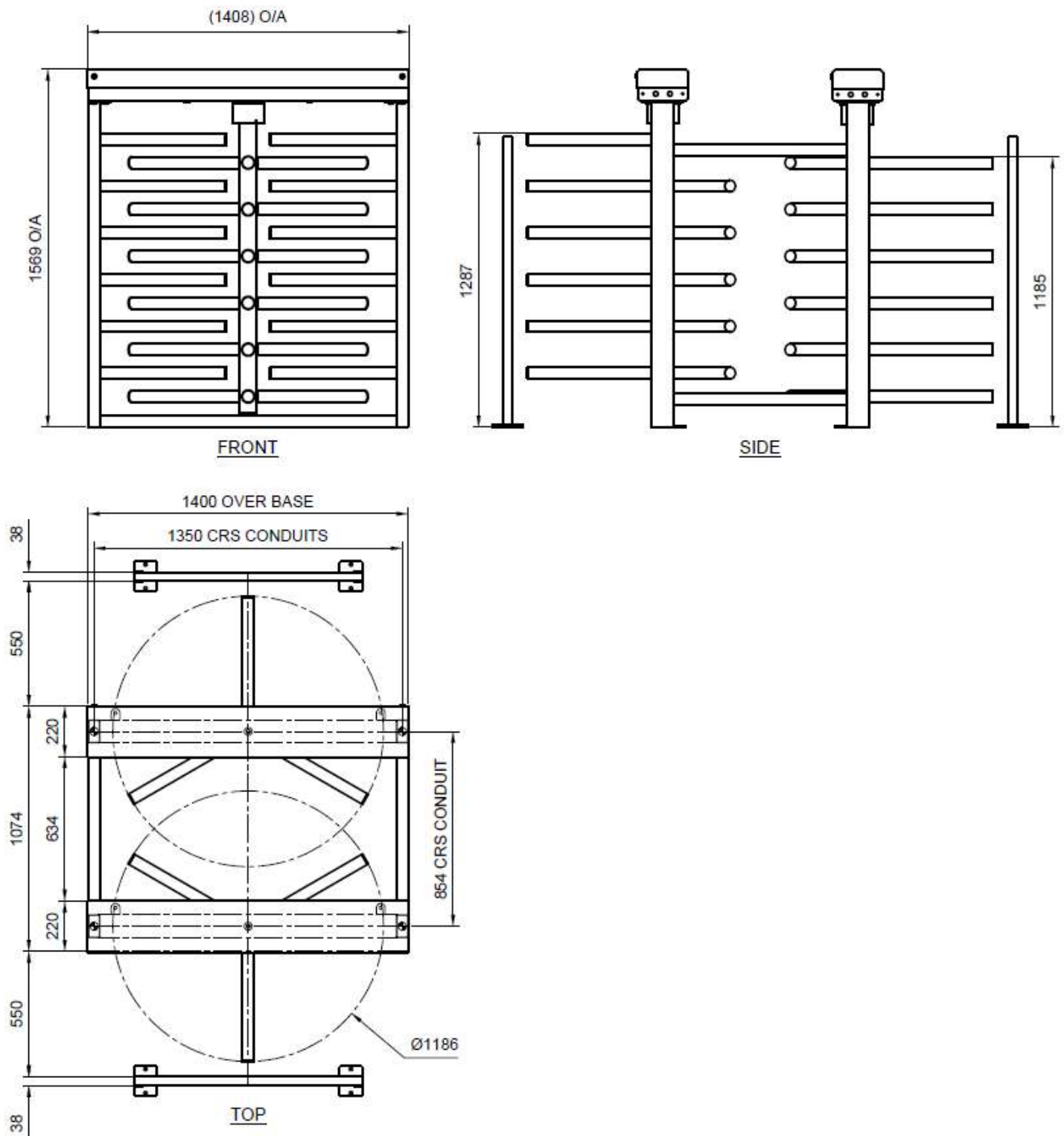
Figure 8: Double 3-Arm Industrial ¾ Height Turnstile
