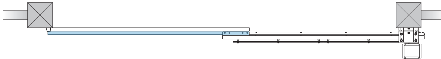
VA5401 Upper guide profile
